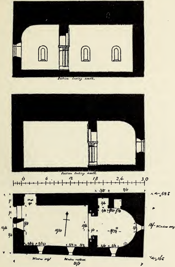
Plan of St. Margaret's Chapel. By Sir Henry Dryden.
