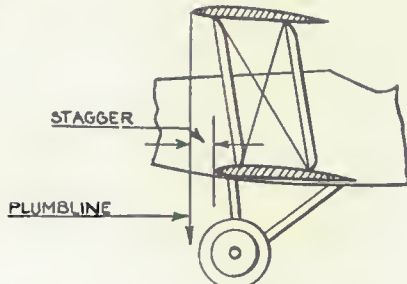
FIG. 8. MEASURING STAGGER
