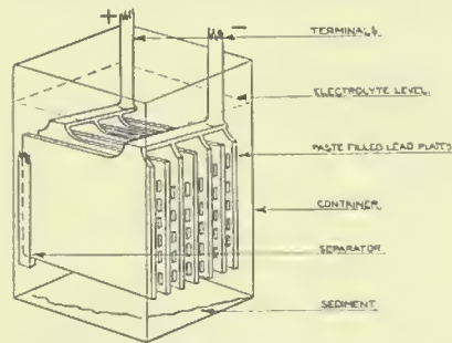
CONSTRUCTION OF MULTIPLE PLATE CELLS
