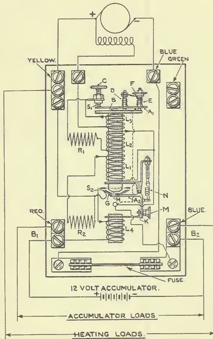
FIG. 75. VOLTAGE CONTROL BOX— DIAGRAM OF CONNECTIONS
