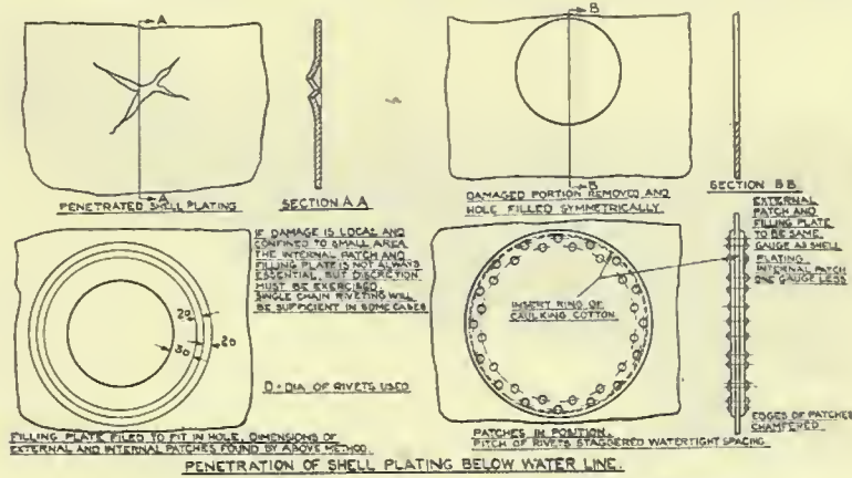
FIG. 47. REPAIRS TO HULLS AND FLOATS BELOW WATERLINE
