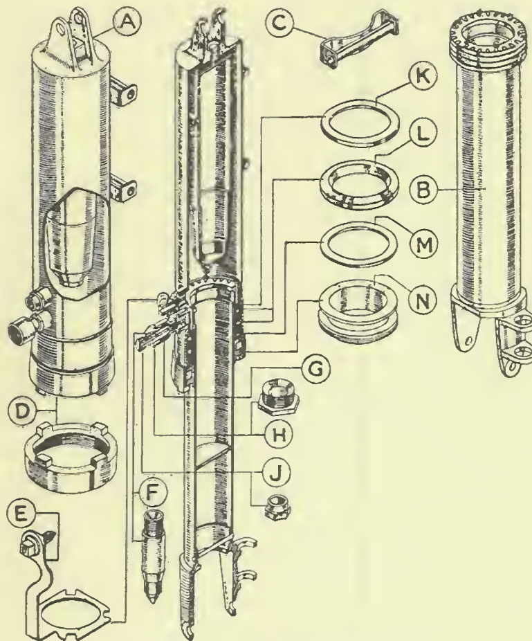
FIG. 39. DETAILS OF OLIO-PNEUMATIC LEG
