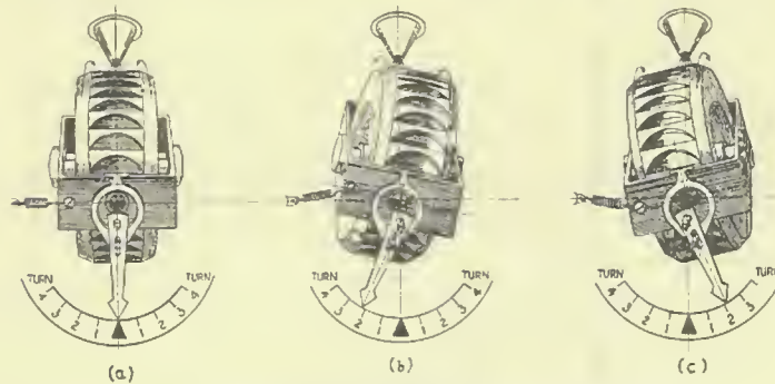
FIG. 66. TURN INDICATOR GYRO ROTOR UNIT
