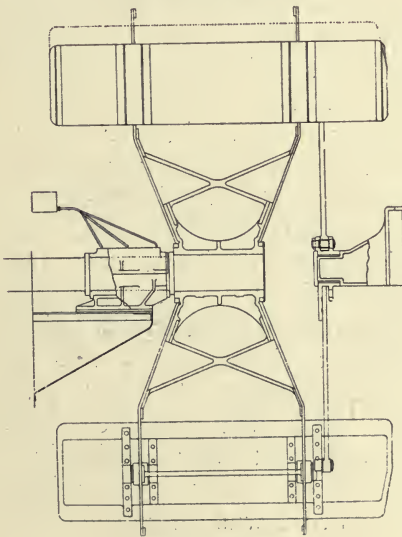
PADDLE WHEEL
