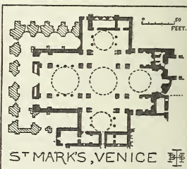
FIGS. 27 AND 28.—SECTION AND PLAN OF ST. MARK'S.
