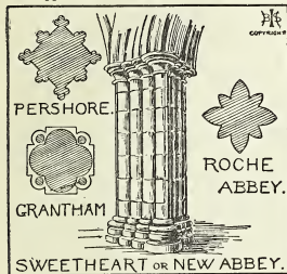
FIG. 45.—PIER TYPES.
