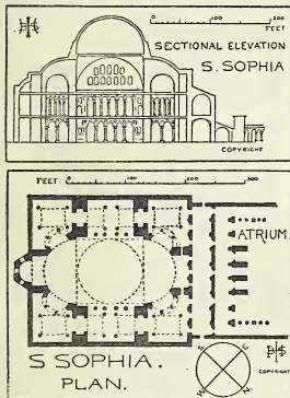
FIGS. 23 AND 24.—SECTION AND PLAN OF ST. SOPHIA.
