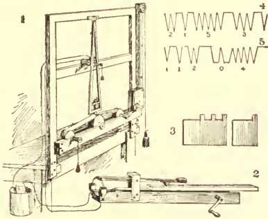
MORSE PENDULUM INSTRUMENT - 1837
