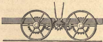
THE SPUR-GEAR.
