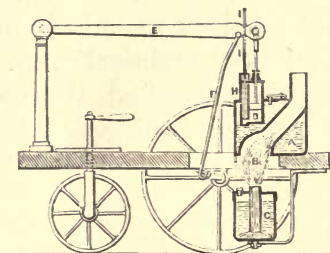
SECTION OF MURDOCK'S MODEL.
