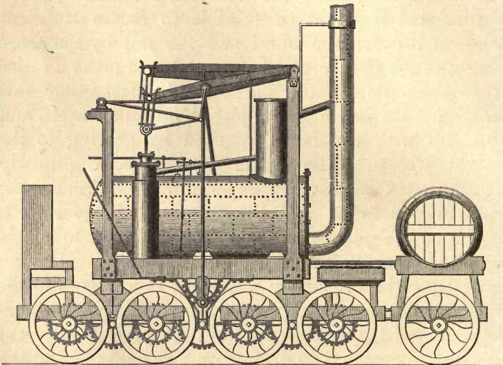
WYLAM ENGINE.
