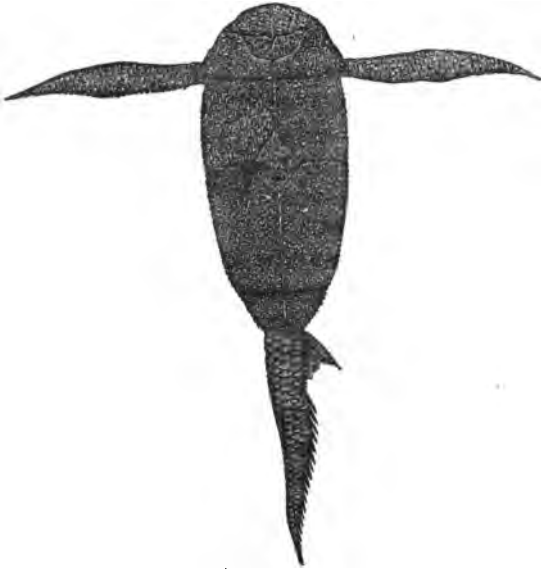
PTERICHTHYS OBLONGUS. One-half nat. size.
