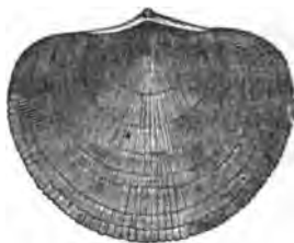
ASAPHUS CAUDATUS. OETHOCERAS LATERALE. SPIRIFERINA RETICULARIS. (Silurian.) (Mountain Limestone.) (Old Red Sandstone.)
