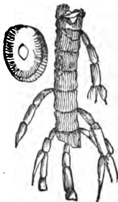
CALAMITES MOUGEOTII.
