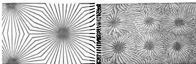
SMITHIA PENGELLYI. (Old Red Sandstone.)
