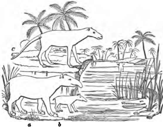
ANIMALS OF THE PARIS BASIN.* (Eocene.)
