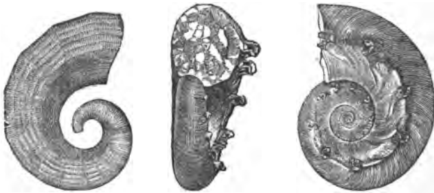
WHORLED SHELLS OF THE OLD RED SANDSTONE.*
