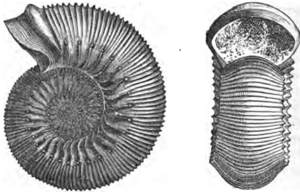
AMMONITES HUMPHRIESIANUS. (Oolite.)
