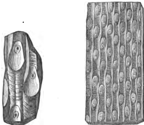
SIGILLARIA GRESERI. ( Coal Measures. )
