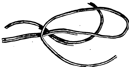
PALÆOCHORDA MINOR. (One-half nat. size.)
