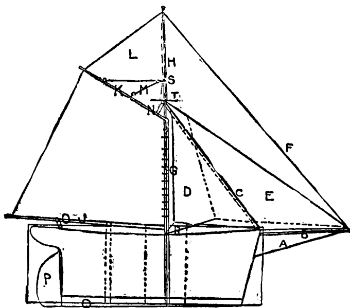
A CUTTER.
