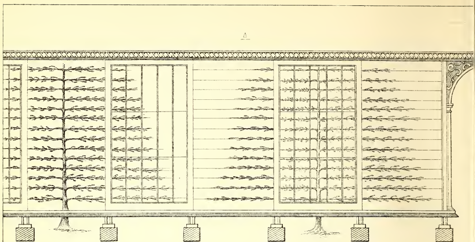
Elevation class A showing alternate sashes open.
