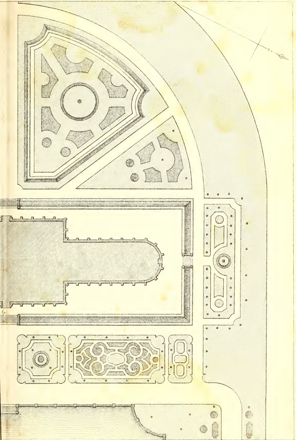
PALM STOVE AT KEW. Plan surrounding it.
