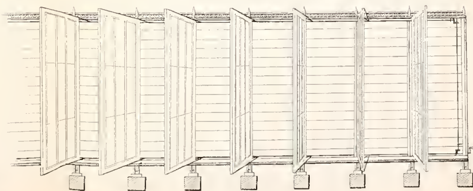
FIG. 7 showing apparatus for opening & shutting doors.
