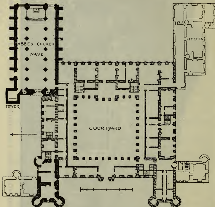
FIG. 2.—PLAN OF GROUND FLOOR, HOLYROOD PALACE.
