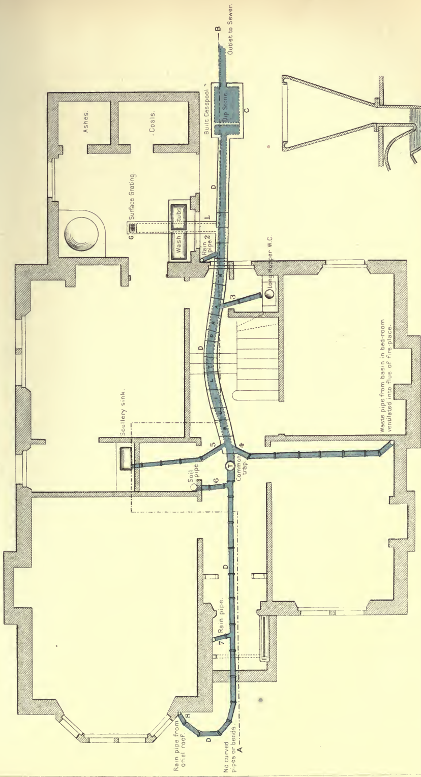
Fig. 1. GROUND PLAN.
