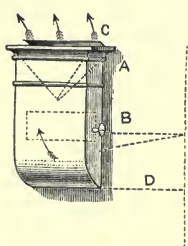
Fig. 273.—Wall Bracket Inlet on Tobin's System.
