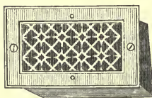
Fig. 276.—Mica-flap Outlet Ventilator (front view).
