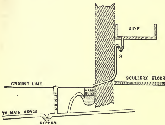
Fig. 293.—Arrangement of Waste-pipe from Scullery Sinks.
