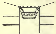
Fig. 290.—Liverpool Bell-trap.
