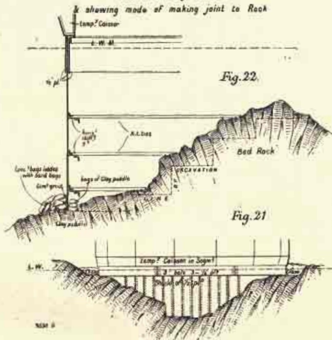
INCH-GARVIE IRON COFFER-DAM, N.W. PIER. Outside view of Shield. BEARING OF CAISSONS ON ROCK FOUNDATIONS.
