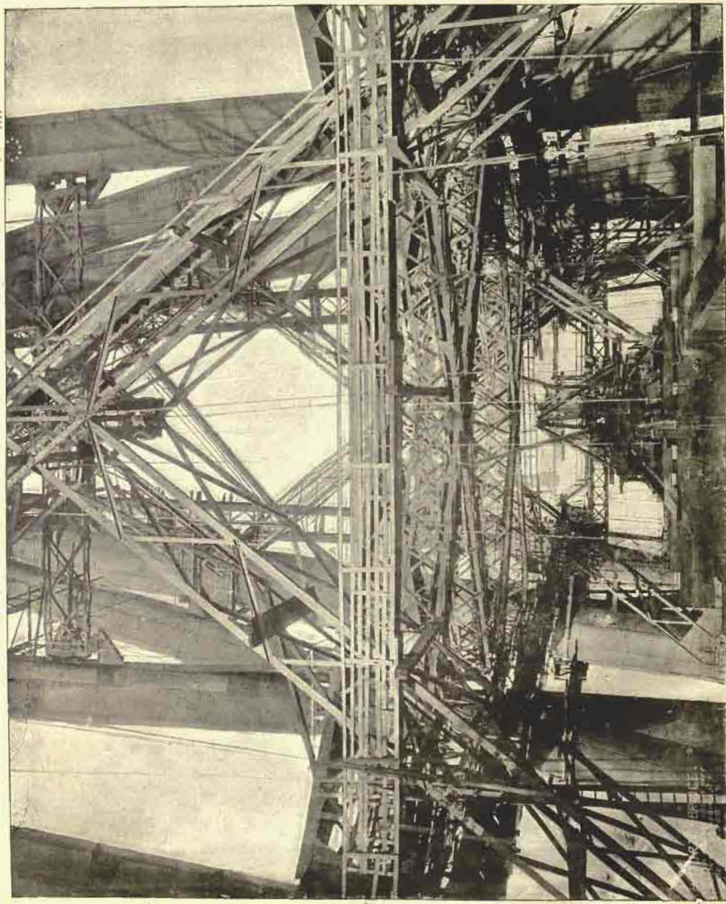
CENTRAL TOWER, QUEENSPERRY PIER; HORIZONTAL AND DIAGONAL BRACING GIRDERS; PART OF INTERNAL VIADUCT AND TEMPORARY STAGING.
