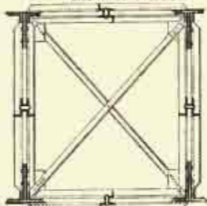
Fig. 118. Cross Section of Inclined Ties in Cantilevers.
