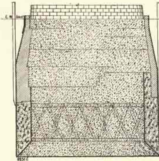
FIG. 47. SECTION OF TILTED CAISSON AFTER COMPLETION.
