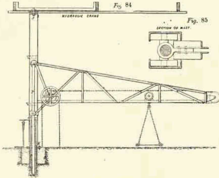
HYDRAULIC CRANES.
