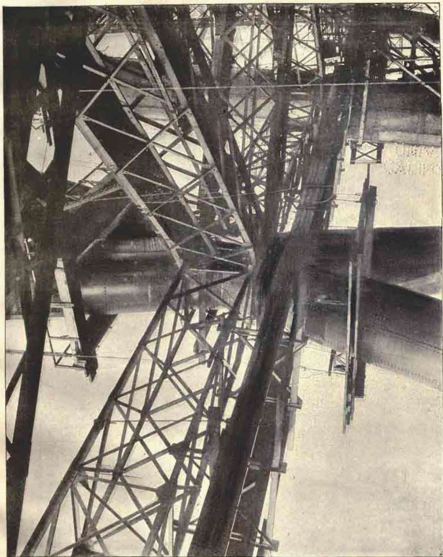
QUEENSFERRY FIER. INTERSECTION OF DIAGONAL STRUTS, WITH HORIZONTAL AND DIAGONAL BRACING GIRDERS.
