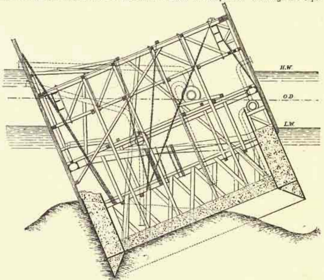
FIG. 46. TILTED CAISSON AT SOUTH QUEENSFERRY.
