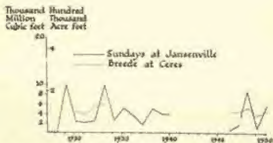
Fig. 46. Annual discharge, Sundays and Breede rivers.
