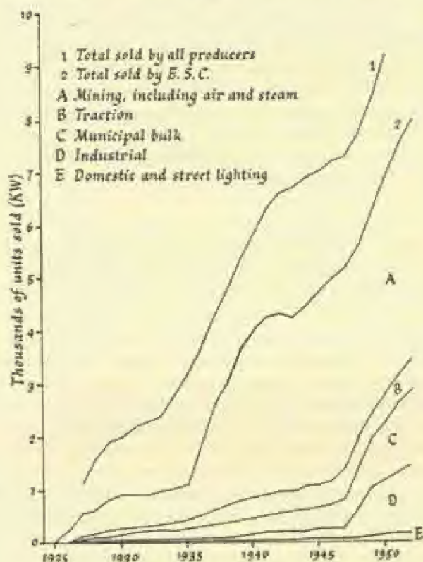
Fig. 141. Electricity consumption, 1925-52.
