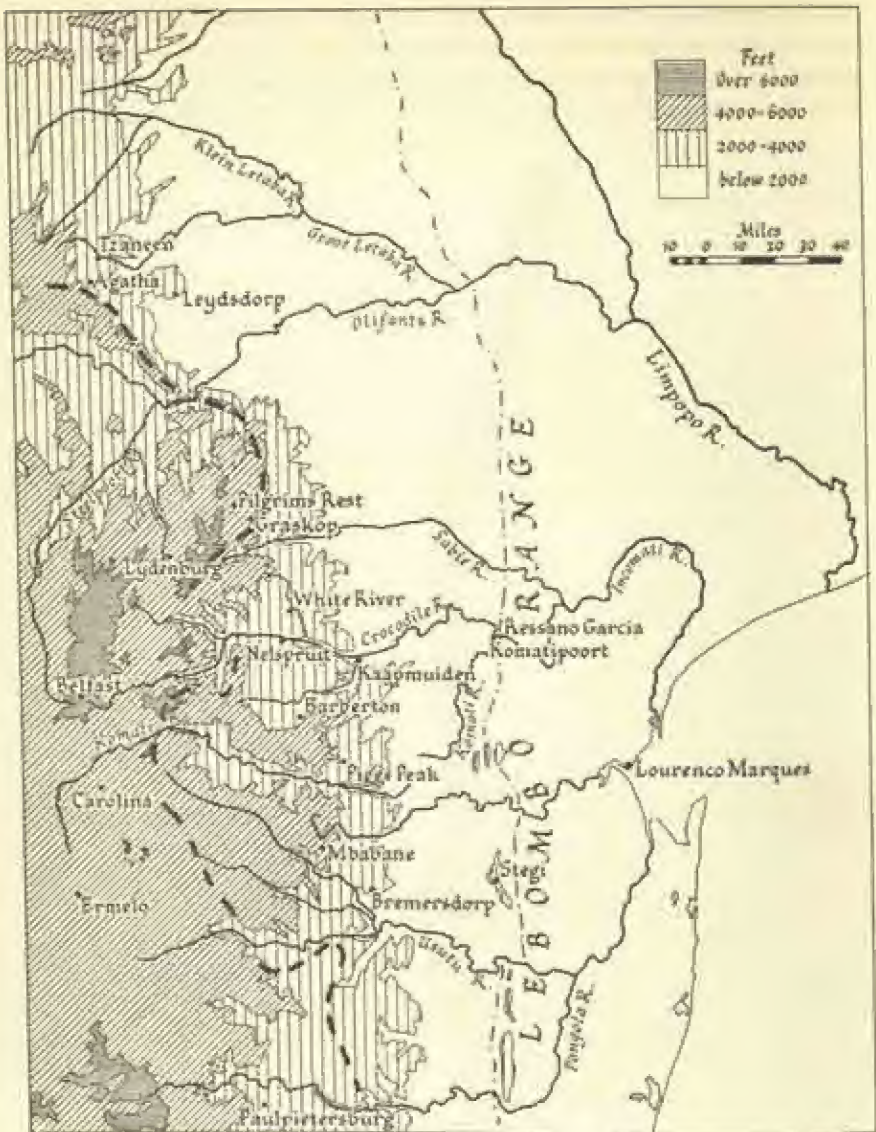
Fig. 207. The Lowveld; topography.
