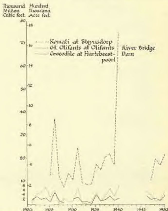
Fig. 44. Annual discharge, Limpopo and Crocodile-Komati river systems. (Compiled from data given in the annual reports of the Director of Irrigation.)
