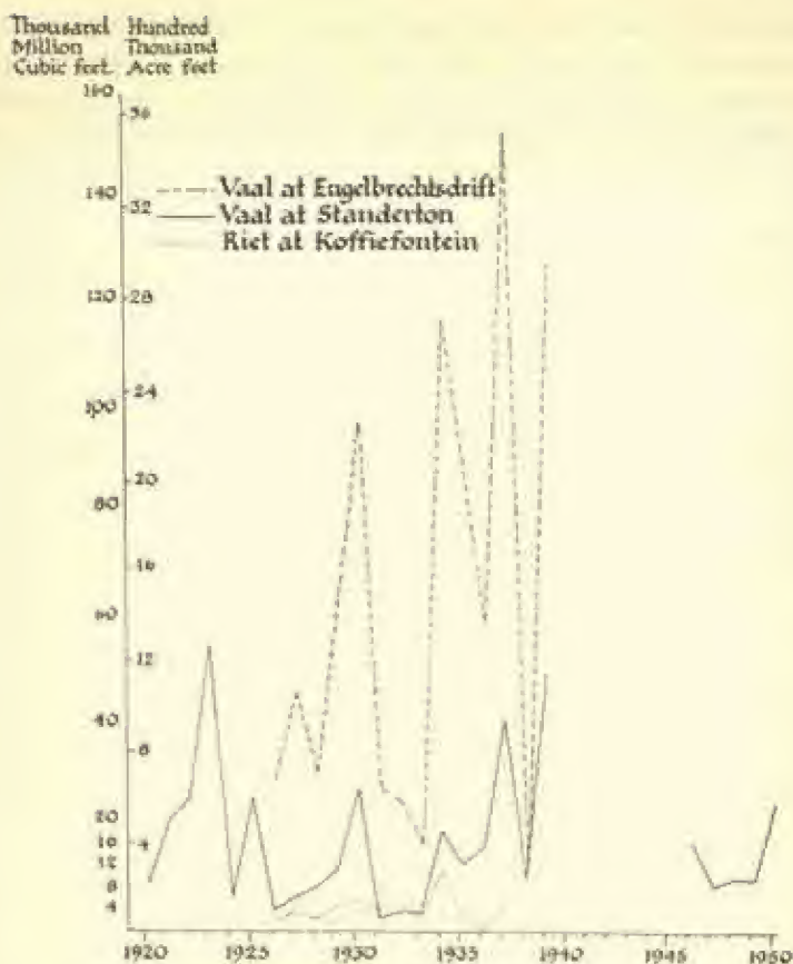
Fig. 45. Annual discharge Orange-Vaal river system.
