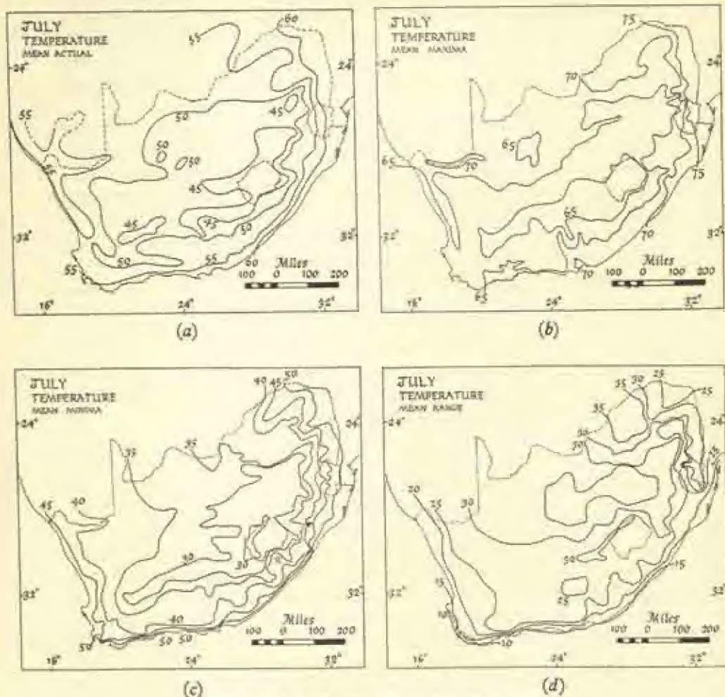
Fig. 26a-d. Temperature conditions in July.
