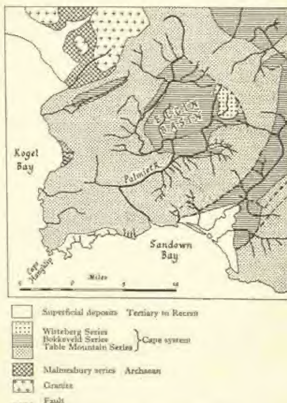
Fig. 189a. The Elgin Basin; geology and drainage.
